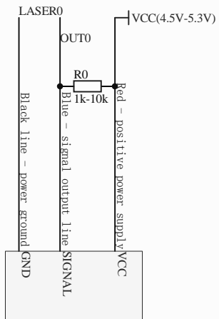
Laser sensors
