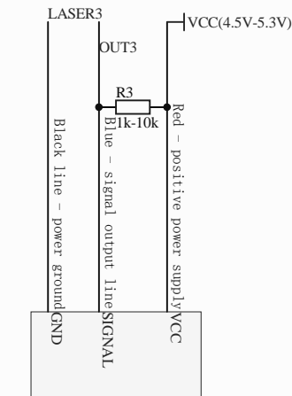
Laser sensors
