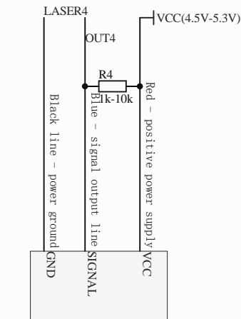
Laser sensors
