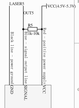
Laser sensors
