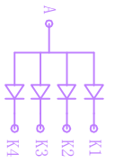
Back Light Circuit
